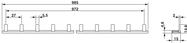
Dimensional drawing
